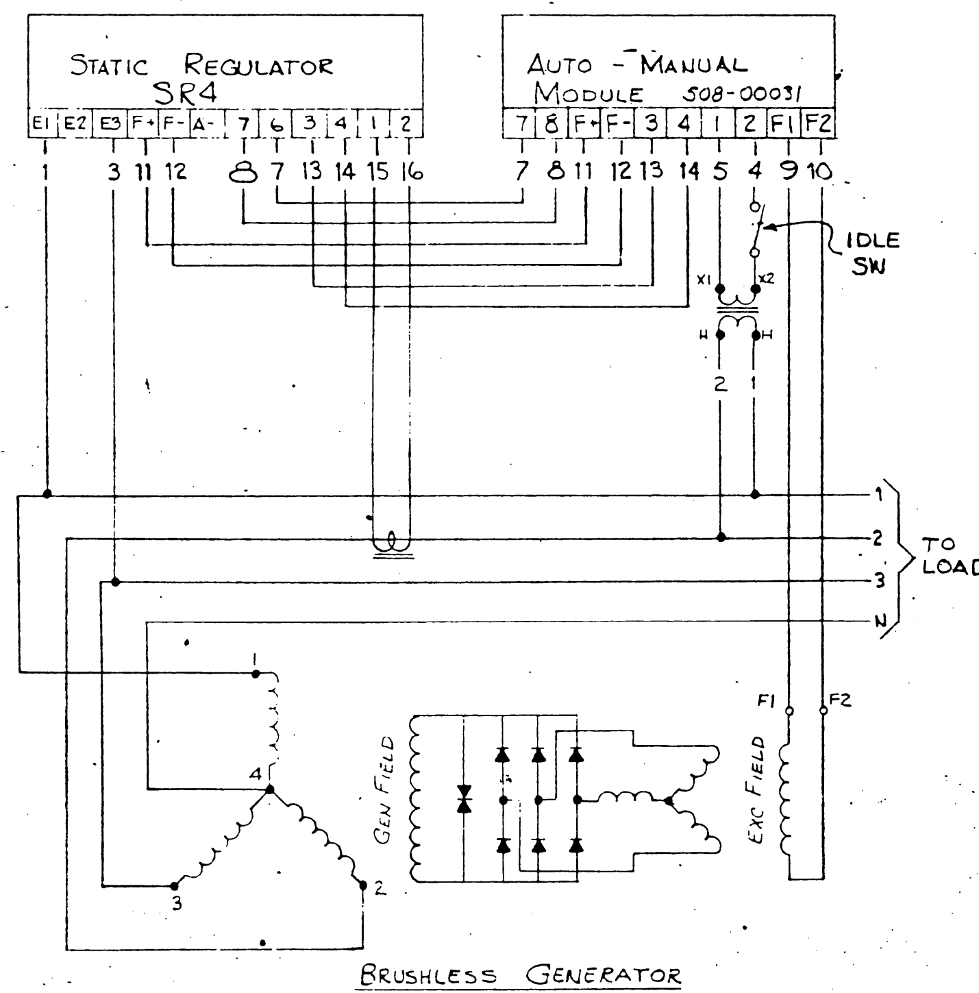
VOLTAGE REGULATOR CONNECTIONS
